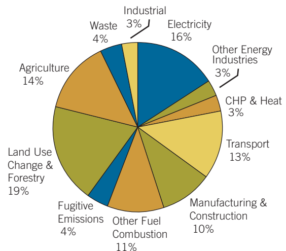
Global GHG Emissions by Sector, 2000
